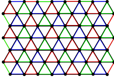
Figure 2: The triangular lattice is covered by three tessellations, which is the minimum number of tessellations required to cover the graph.
