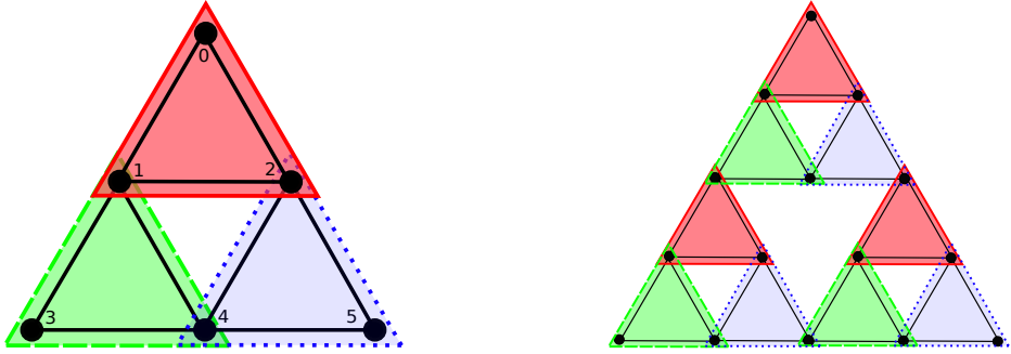
Figure 1: (Left) The Hajós graph S_2 . (Right) The Sierpiński Sieve graphs can always be covered by three tessellations. For better visualization, only maximal cliques are depicted here for each tessellation. These graphs cannot be covered by less than three tessellations.
