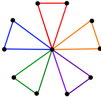
Figure 3: The class of windmill graphs is tight with respect to the upper bound of Theorem 1. The windmill \text{Wd}_{3,5} has 5 triangles, its clique graph K(\text{Wd}_{3,5}) is the complete graph with 5 vertices, and the tessellation number T(\text{Wd}_{3,5}) is 5.
