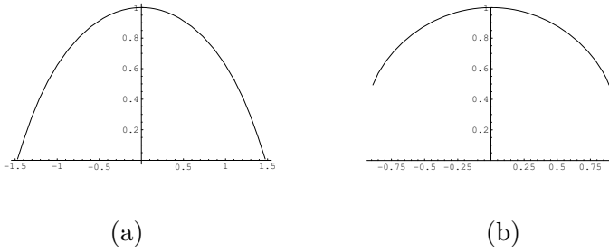
Figure 2: The generating curve of a parabolic surface with aH + bK = 1 , with 0 < a < 1 and a + 2b < 0 . Here z_0 = 1 and a = 0.5 . In the case (a), b = -1 and in the case (b), b = -0.8 .
