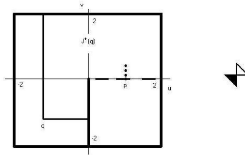
Figure 1: \mathbb{L}^2 , g = -2dudv , M open subset (Remark 3.10(2)), which is stably causal. J^+(q) is not closed at q = (-1, -1) , and t^- is not continuous at p = (1, 0) .
